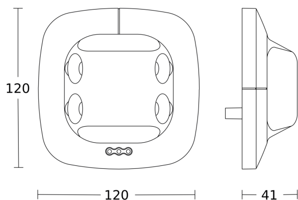
Dimension Drawing 1
